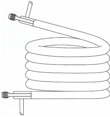
Fig. 3 Schematic of a Double pipe (tube-in-tube) type condenser & shell & coil type condenser used in small refrigeration systems.
