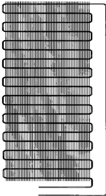
Fig. 1. Finned tube condenser used for experimental and theoretical study
