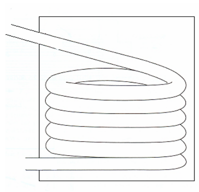
Fig. 3 Schematic of a Double pipe (tube-in-tube) type condenser & shell & coil type condenser used in small refrigeration systems.
