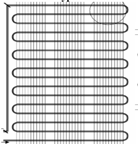
Fig. 2 Schematic of a wire-and-tube type & plate fin type condenser r used in small refrigeration systems
